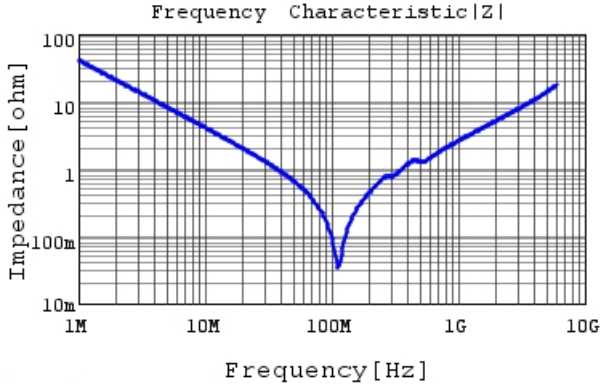
GCM2165C1H392JA16 |Z| DCOV,25degC
