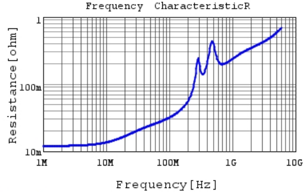
GCM2165C1H392JA16 R DCOV,25degC
