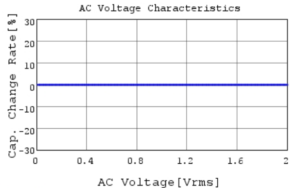
GCM2165C1H392JA16 C-AC Voltage capchange, D
