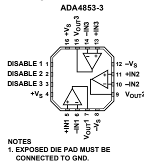
Figure 3. 16-Lead LFCSP_WQ
