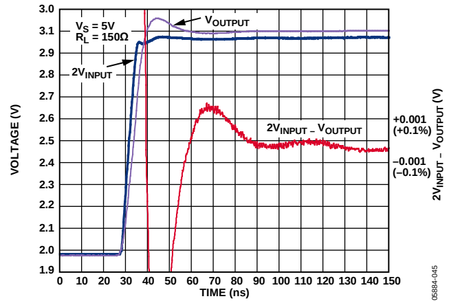
Figure 46. 0.1% Settling Time
