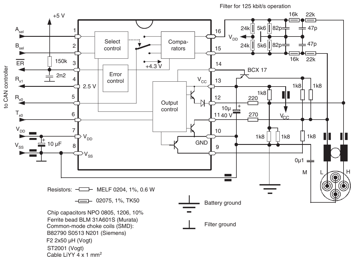
Figure 6-2. Application Circuit
