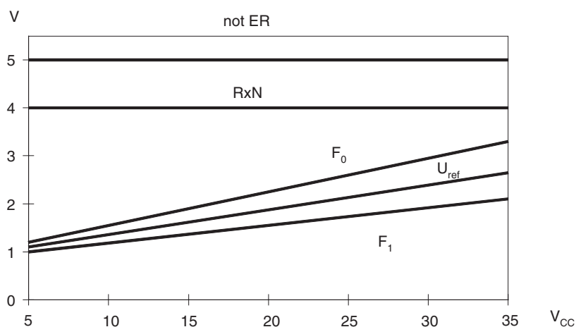
Figure 7-1. Comparator Thresholds
