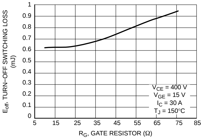
Figure 13. Switching Loss vs. R_G
