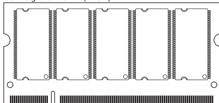
Figure 1: Low-Profile Layout
