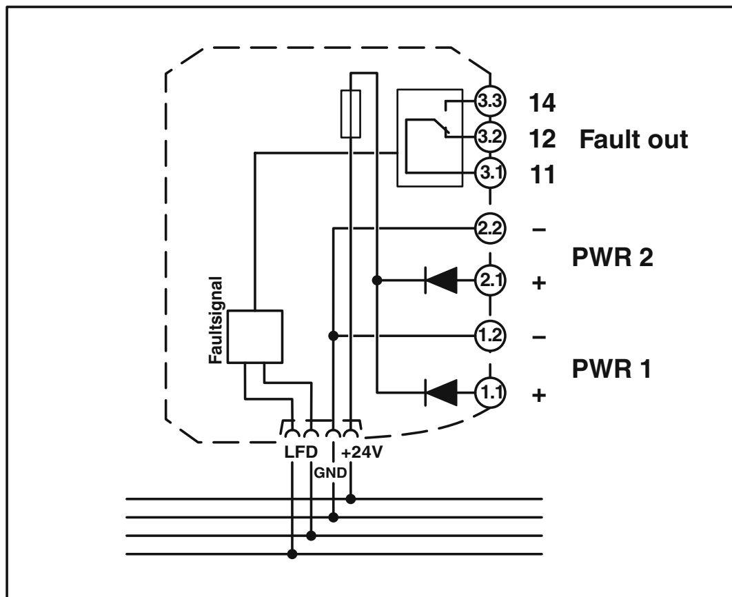
Block diagram
