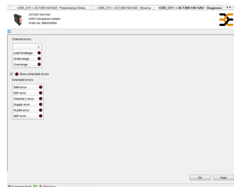
Screenshot diagnosis with FDT/DTM software
