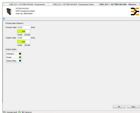
Screenshot of observe with FDT/DTM software
