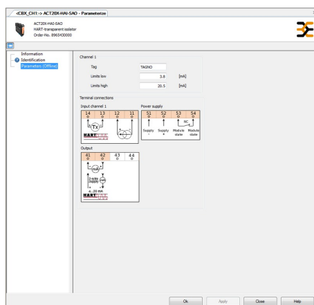
Screenshot of input configuration with FDT/DTM software
