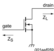
Fig 19. Definition of transistor impedance
