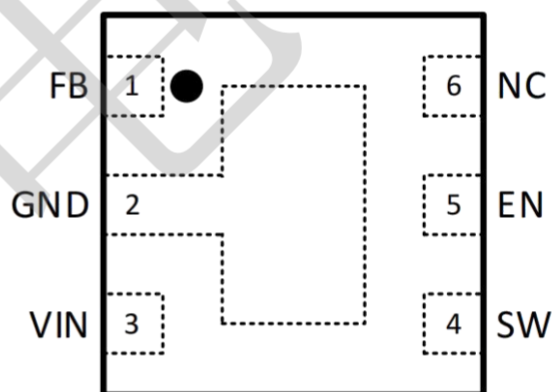
DFN-6(1.6X1.6)
