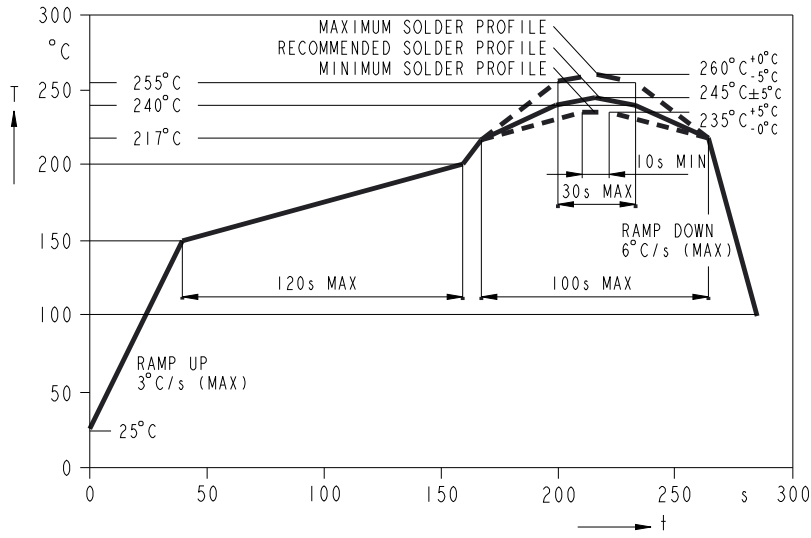
RoHS COMPLIANT REFLOW PROFILE
