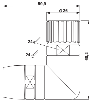
Dimensional drawing
