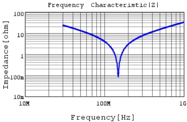
RCE5C2J221J1K1H03B |Z| DCOV, 25degC
