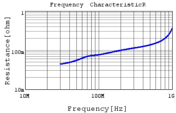
RCE5C2J221J1K1H03B R DCOV, 25degC
