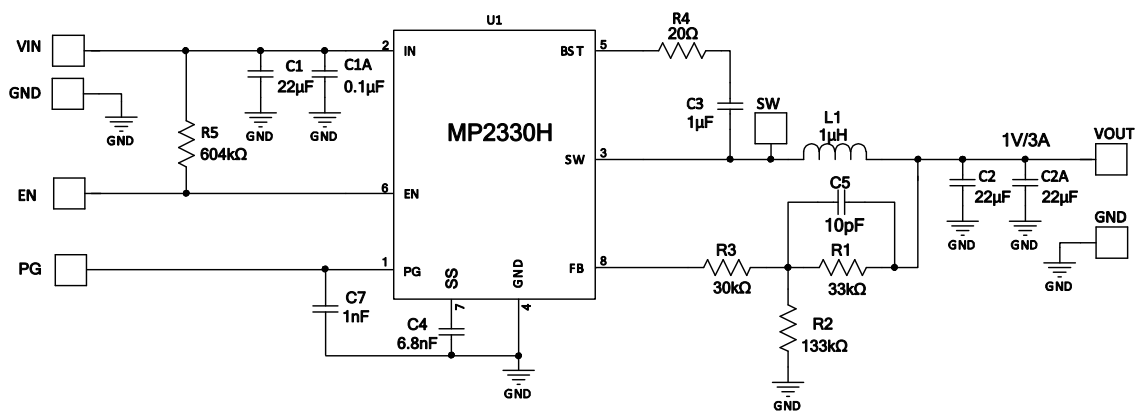
Figure 12: V_{IN} = 19V , V_{OUT} = 1V/3A
