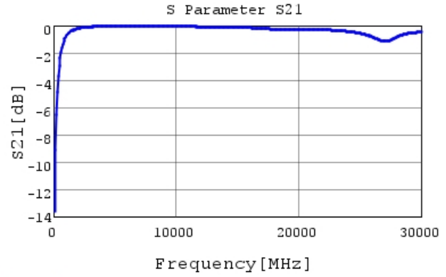
GRM0225C1C3R4BA03 S21 DCOV, 25degC
