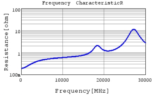
GRM0225C1C3R4BA03 R DC0V, 25degC
