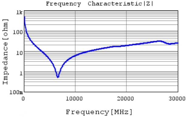
GRM0225C1C3R4BA03 |Z| DC0V, 25degC
