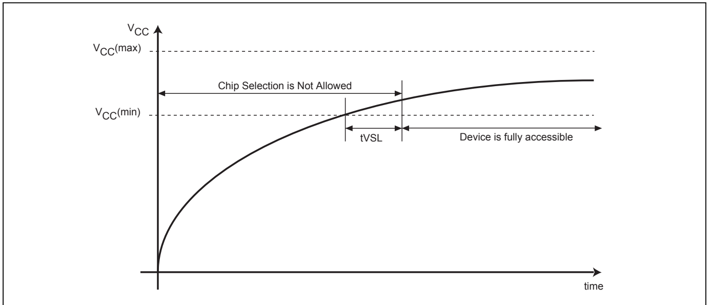
Figure 27. Power-up Timing
