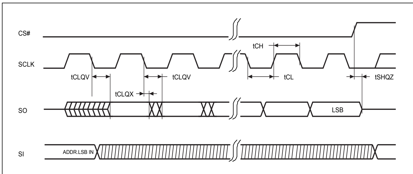
Figure 8. Output Timing
