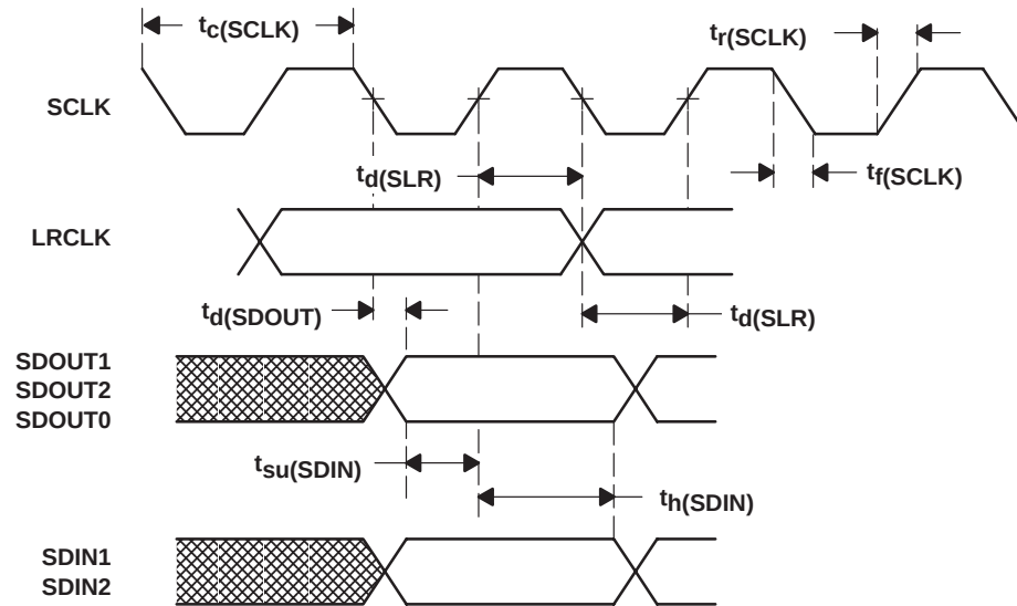
Figure 2–2. For Right/Left Justified, I²S, Left/Left Justified Serial Protocols
