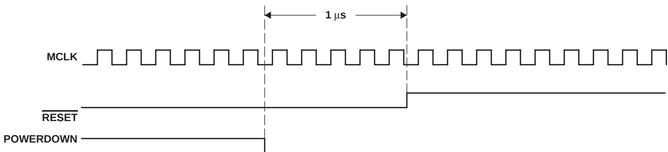
Figure 5–3. Start-Up Timing
