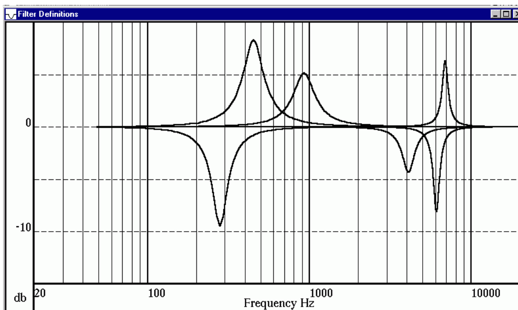
Figure 8–6. Equalization Filters
