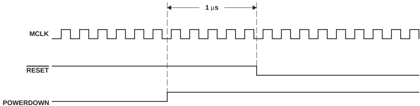
Figure 5–2. Power-Down Timing
