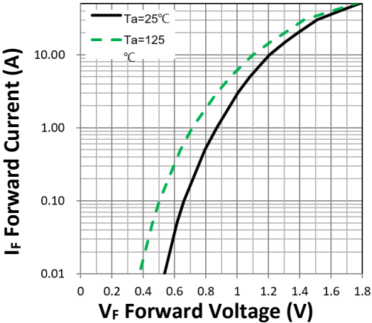
Figure 1. Forward Characteristic(typ.)
