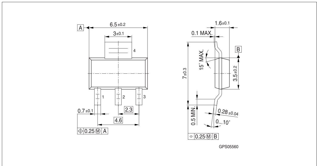
Figure 1 SOT 223
