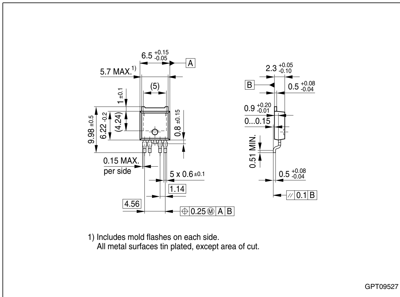
Figure 4 PG-TO252-5-11 (Plastic Transistor Single Outline)
