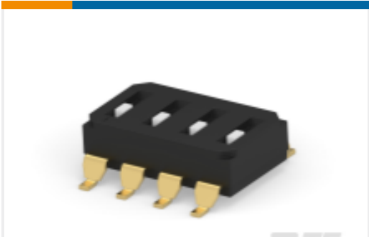
TE Part #4-2319848-6 END STACK DIP 4P G RECESS T&R
