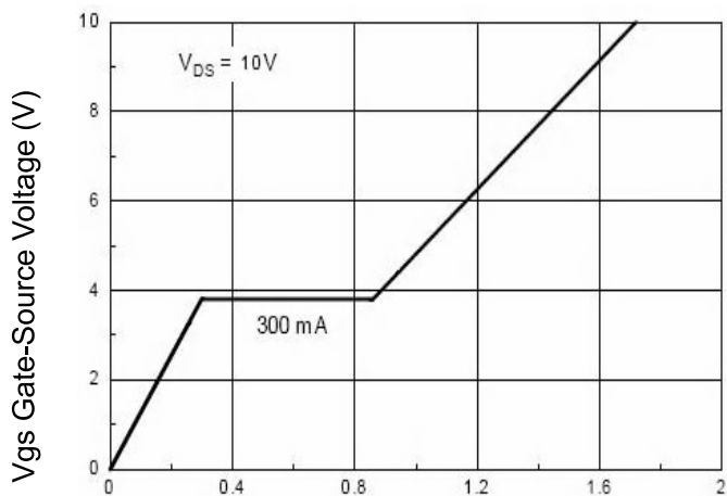
Figure 7 Gate Charge
