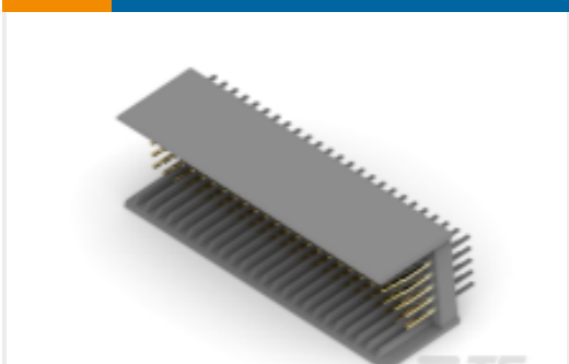
TE Part #3-100141-0 Z-PACK/B MALE HDR 125P, 2MM HM
