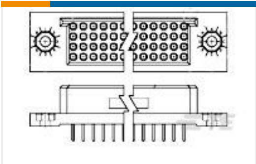
TE Part #533285-6 BOX II 4 ROW RECP ASSY 180 POS
