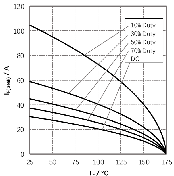
Figure 4. Current Derating
