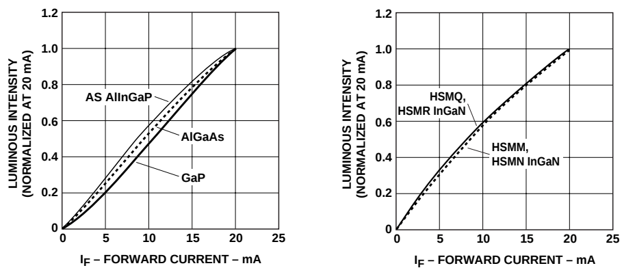
Figure 3. Luminous intensity vs. forward current.
