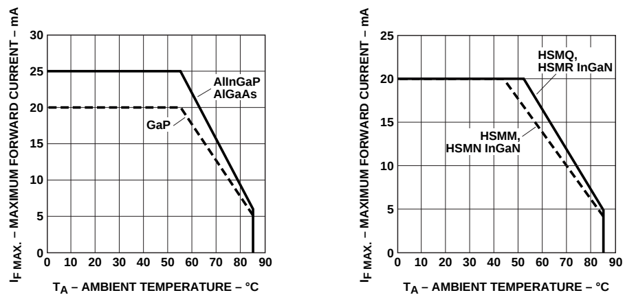
Figure 4. Maximum forward current vs. ambient temperature.
