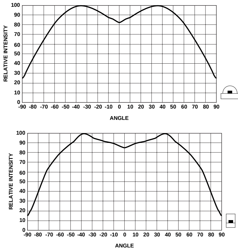
Figure 5. Relative intensity vs. angle.
