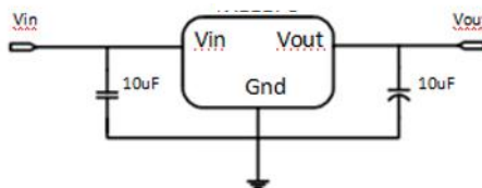
Application circuit of TLV1117-xxIDCYR fixed version
