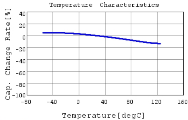
GRM033R71C103ME14 C-Temp. capchange, DC0.0V,
