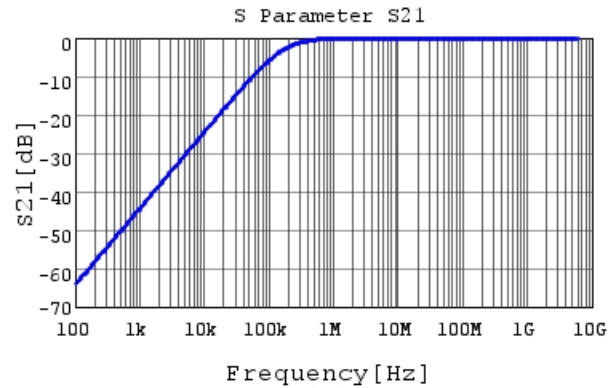
GRM033R71C103ME14 S21 DC0V, 25degC
