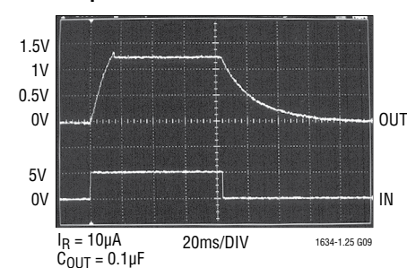
Response Time
