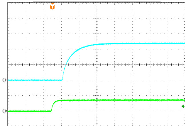
Turn-on transient at full load current (20ms/div). Top Trace: V out ; 5V/div; Bottom Trace: ON/OFF input: 5V/div.
