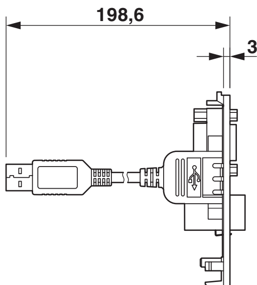
Dimensional drawing
