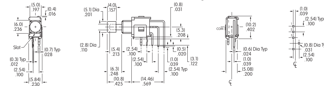
AB11 model does not have terminal 2. AB15AV-FA
