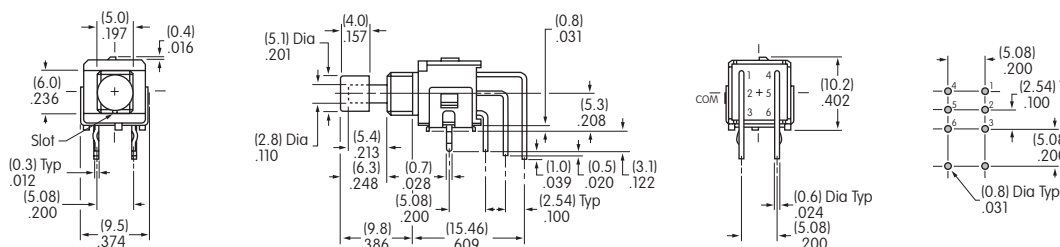
AB11 model does not have terminal 2. AB15AV-FA
