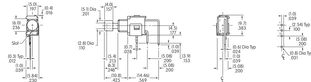
AB11 model does not have terminal 2. AB11AV1-FA
