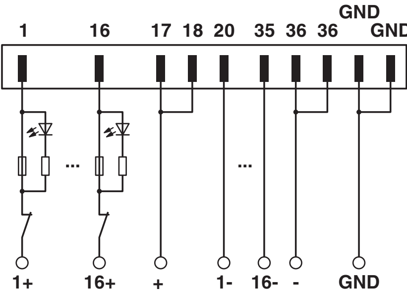
Circuit diagram
