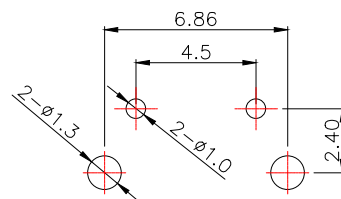
RECOMMEND P.C.B LAYOUT PCB TOLERANCE:±0.05 (TOP VIEW)
