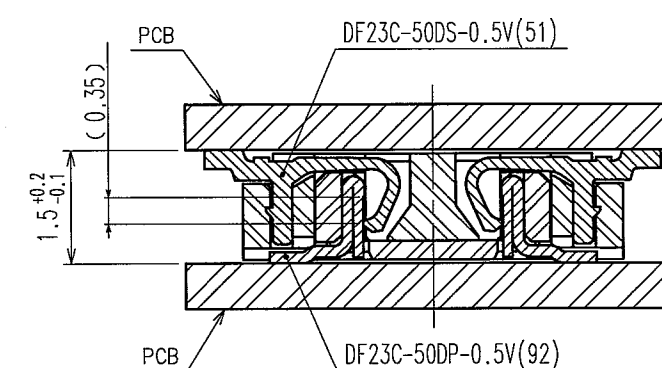
Fig.4 : MATING VIEW
