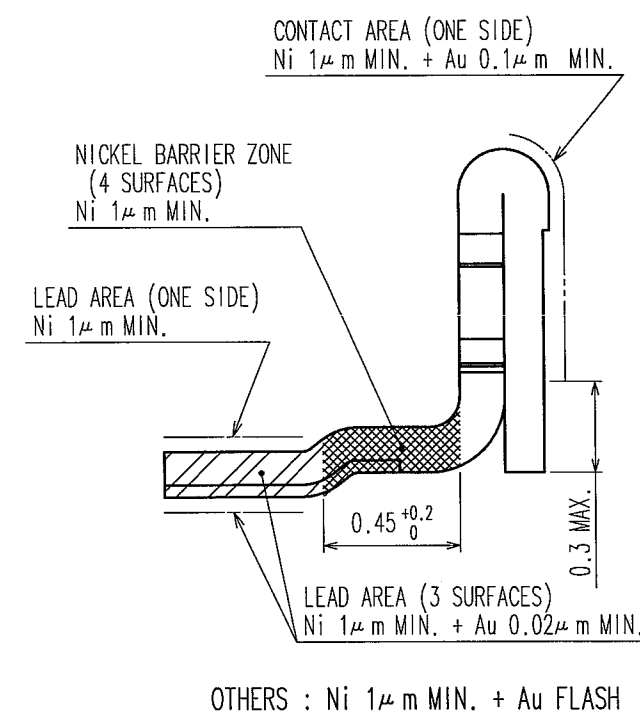
Fig.4 : MATING VIEW
