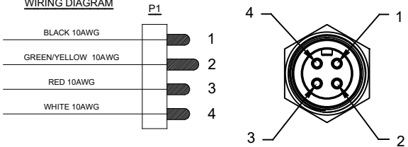
WIRING DIAGRAM
