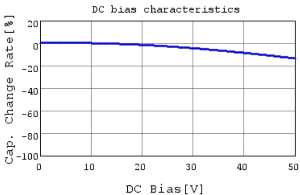
RHEL81H472K0DBH03A C-DC bias capchange, 25.0
