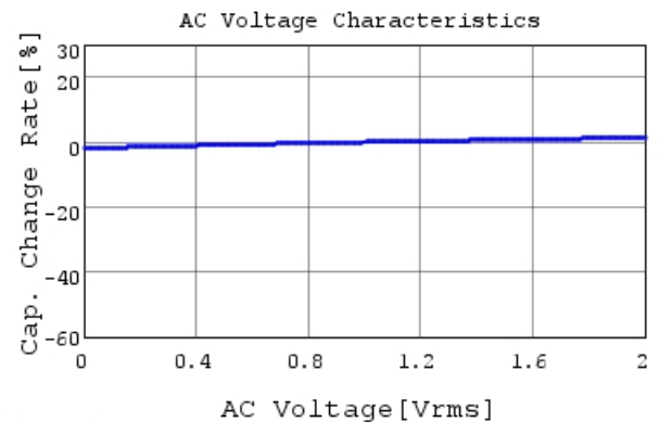
RHEL81H472K0DBH03A C-AC Voltage capchange, 1
