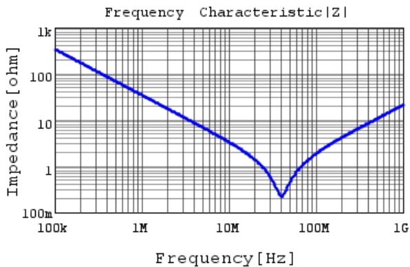
RHEL81H472K0DBH03A |Z| DCOV, 25degC
