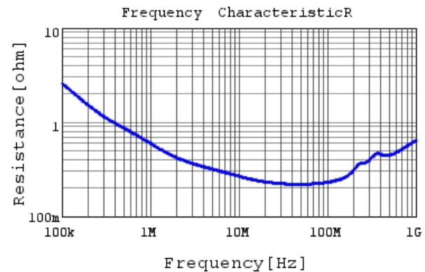
RHEL81H472K0DBH03A R DCOV, 25degC
