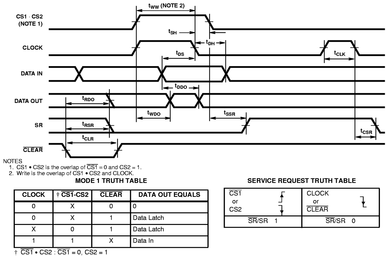
FIGURE 6. MODE 1 OUTPUT PORT TIMING WAVEFORMS AND TRUTH TABLES
