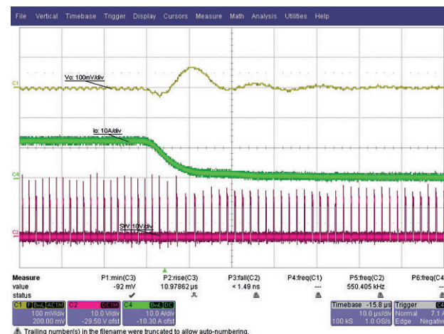
Fig. 33 - Load Release, 12 A to 0.1 A, 1 A/ \mu s, t = 10\text{ }\mu\text{s/div} Forced Continuous Conduction Mode
