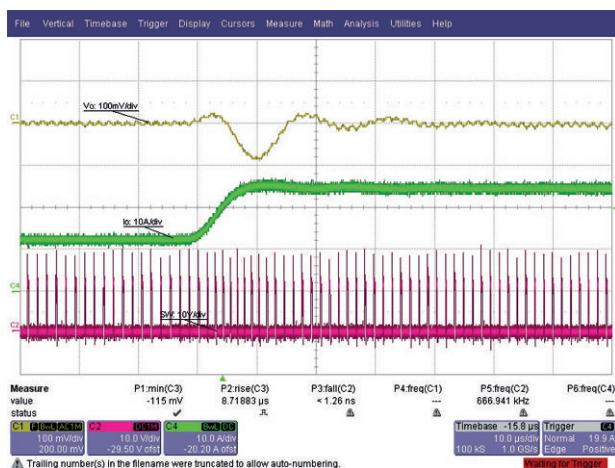
Fig. 28 - Load Step, 12 A to 24 A, 1 A/ \mu s, t = 10\text{ }\mu\text{s/div}
