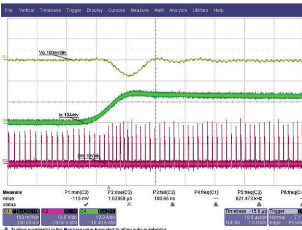
Fig. 30 - Load Step, 0.1 A to 12 A, 1 A/ \mu s, t = 10\text{ }\mu\text{s/div} Forced Continuous Conduction Mode
