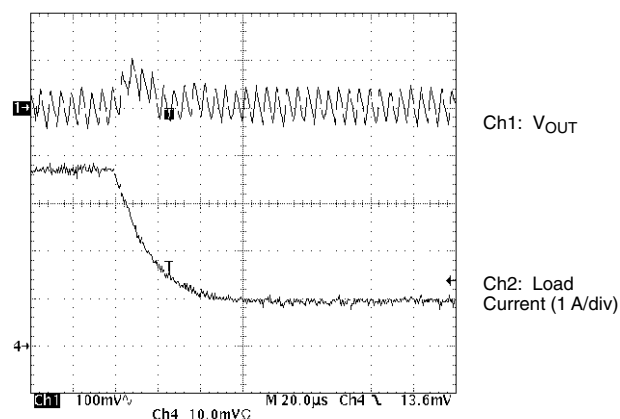
PWM, Unloading 3 V Converter ( V_{IN} = 10 V)
