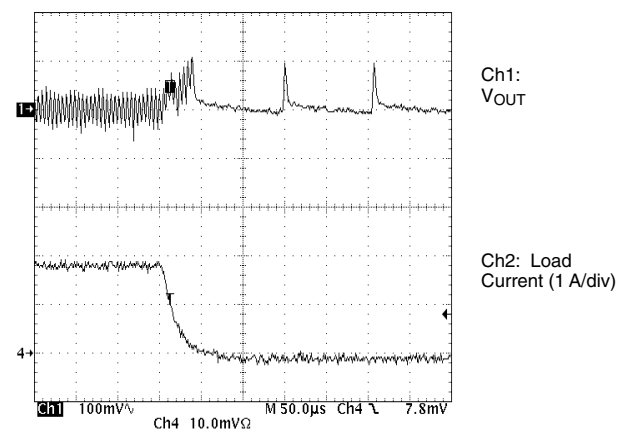
PWM \rightarrow PSM 3 V Converter ( V_{IN} = 10 V)
