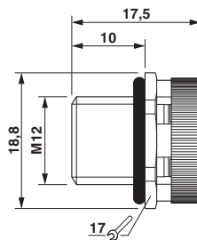
Dimensional drawing
