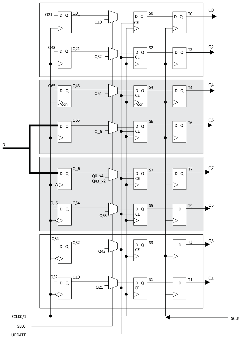
Figure 2.12. Input Gearbox
