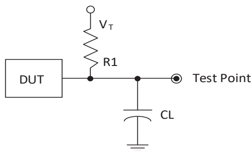
Figure 3.9. Output Test Load, LVTTL and LVCMOS Standards
