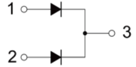
Equivalent Circuit
