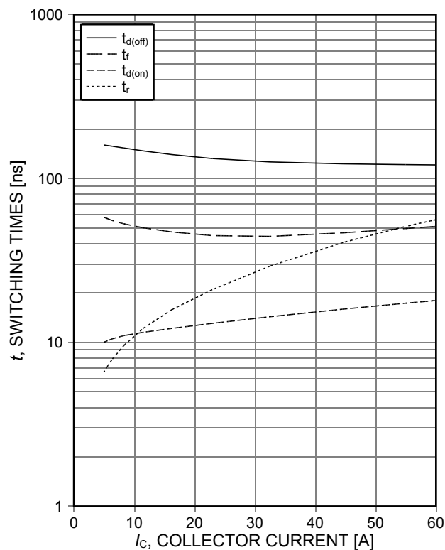
Figure 7. Typical switching times as a function of collector current (inductive load, T_{vj}=150^{\circ}C , V_{CE}=400V , V_{GE}=0/15V , R_G=25\Omega , Dynamic test circuit in Figure E)
