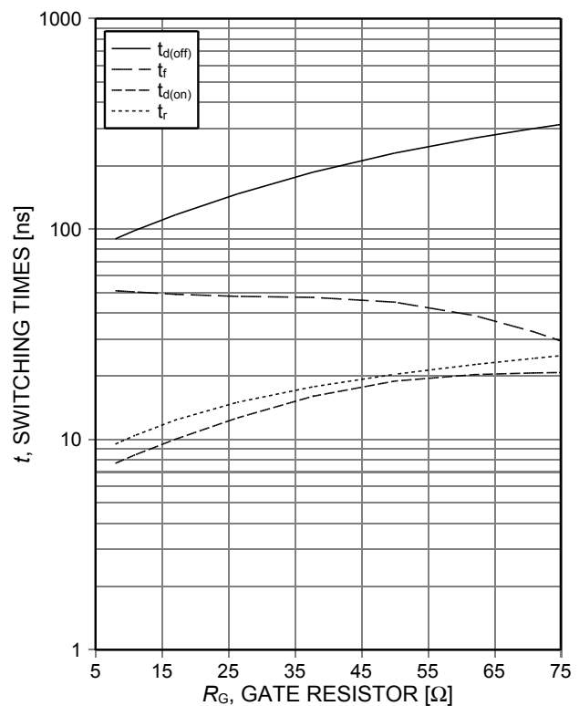
Figure 8. Typical switching times as a function of gate resistor (inductive load, T_{vj}=150^{\circ}C , V_{CE}=400V , V_{GE}=0/15V , I_C=15A , Dynamic test circuit in Figure E)
