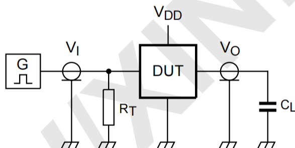
Figure 3. Test circuit for switching times
