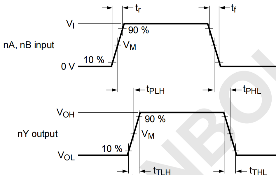
Figure 4. Propagation delay, output transition time
