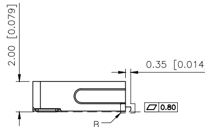
02P~04P Single Hole Scale 1:0.7
