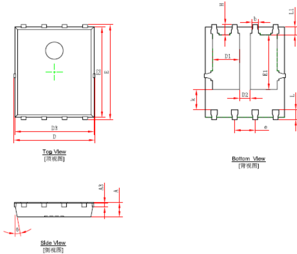
PDFNWB5×6-8L-A PACKAGE OUTLINE DIMENSIONS
