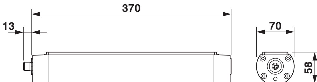
Dimensional drawing
