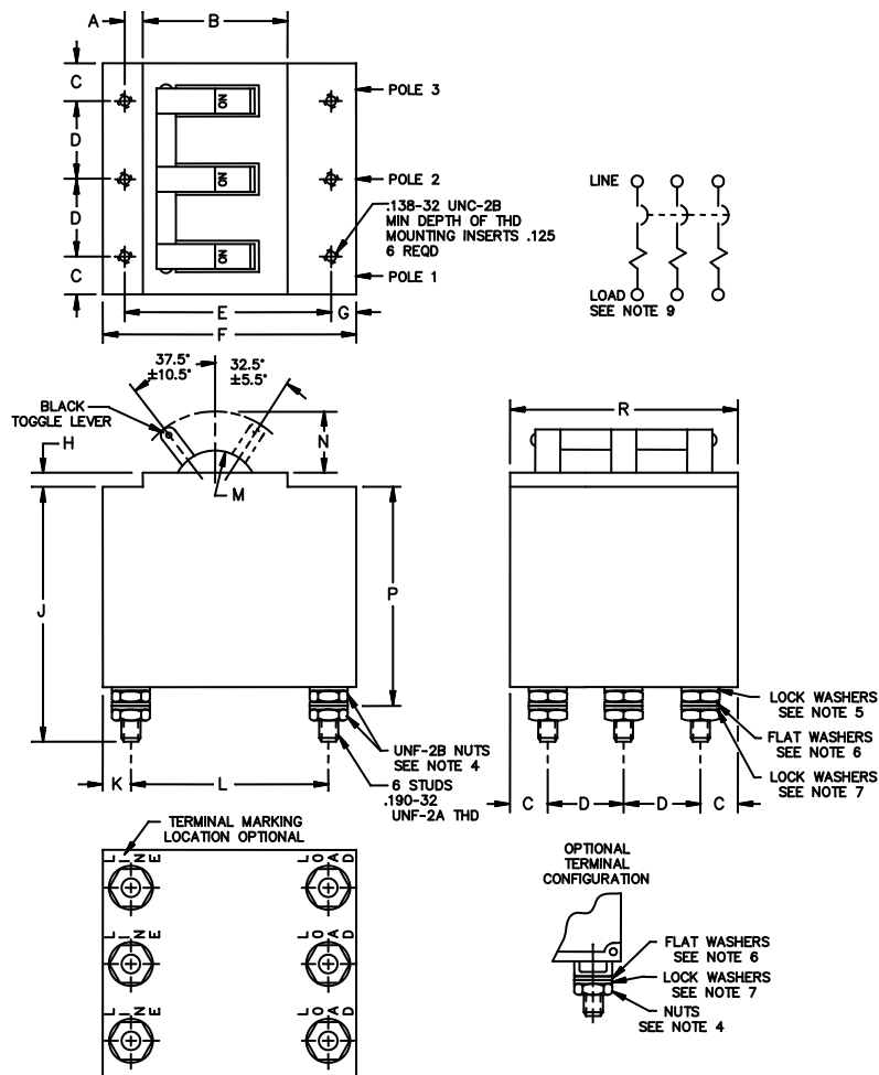
FIGURE 1. Dimensions and configurations (configuration 1).
