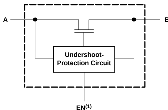
SIMPLIFIED SCHEMATIC, EACH FET SWITCH (SW)
