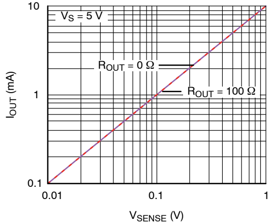
Figure 4. V_{SENSE} vs. Output Current
