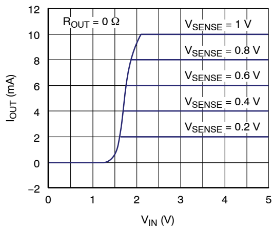
Figure 8. Transfer Characteristics
