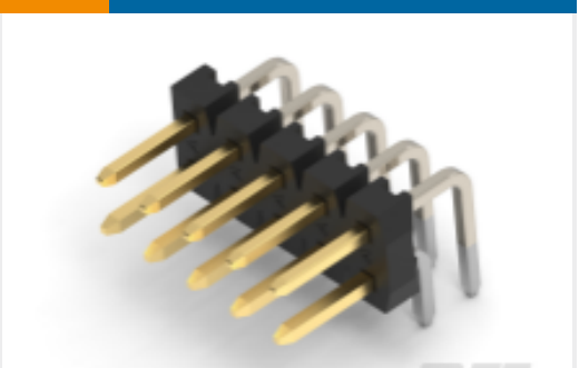
TE Part #2842154-5 10P,2MM,BRK HDR,DRRT,2.8,0.1AU, TB W/CAP
